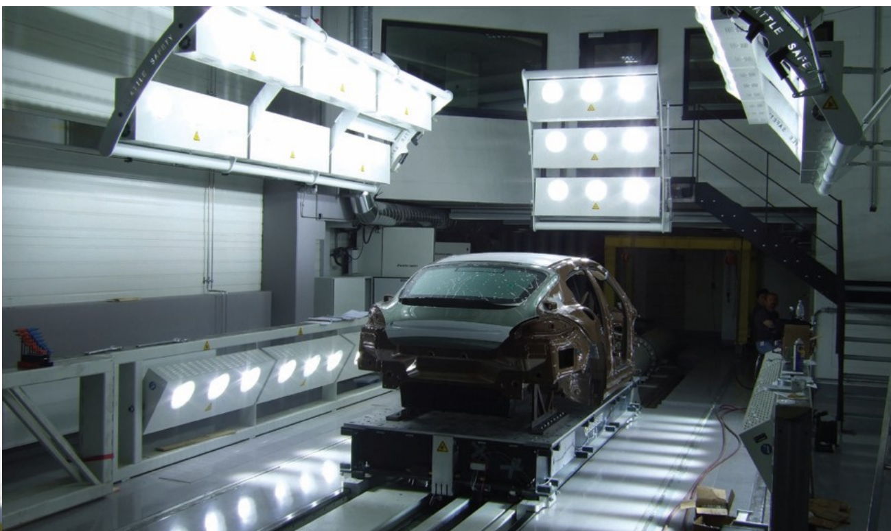
ServoSled ready for NCAP frontal impact testing.
